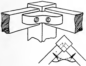
FIG. 394. REINFORCED CORNER.
